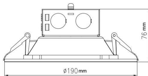
Size : \Phi 190x76mm(7.48x2.99")
